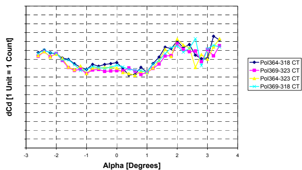
Figure 22 Drag Increment Repeatability at High Reynolds Number
