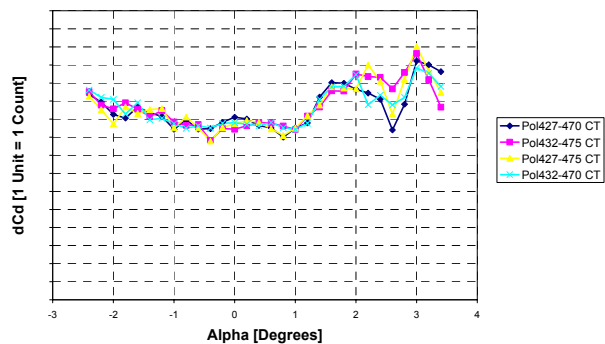
Figure 21 Drag Increment Repeatability at low Reynolds Number
