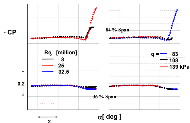
Figure 7 Trailing Edge Pressure Characteristics
