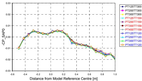
Figure 16 Raw Pressure Distribution along Calibration Probe, All Conditions at Mach 0.85
