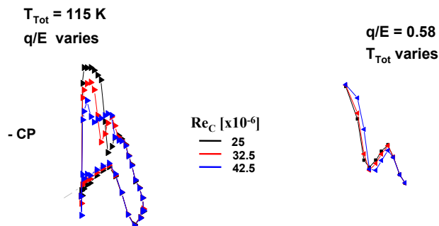
Figure 8 Pseudo and True Reynolds Number Effects on Wing Pressure Distribution
