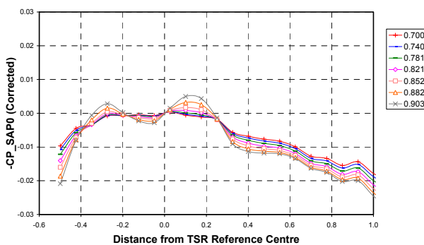
Figure 17 Corrected Pressure Distributions Valid for HiReTT TSR Test Series
