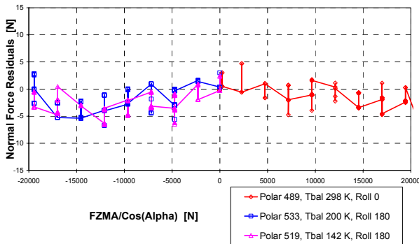
Figure 12 Combined Balance Normal Force Residuals
