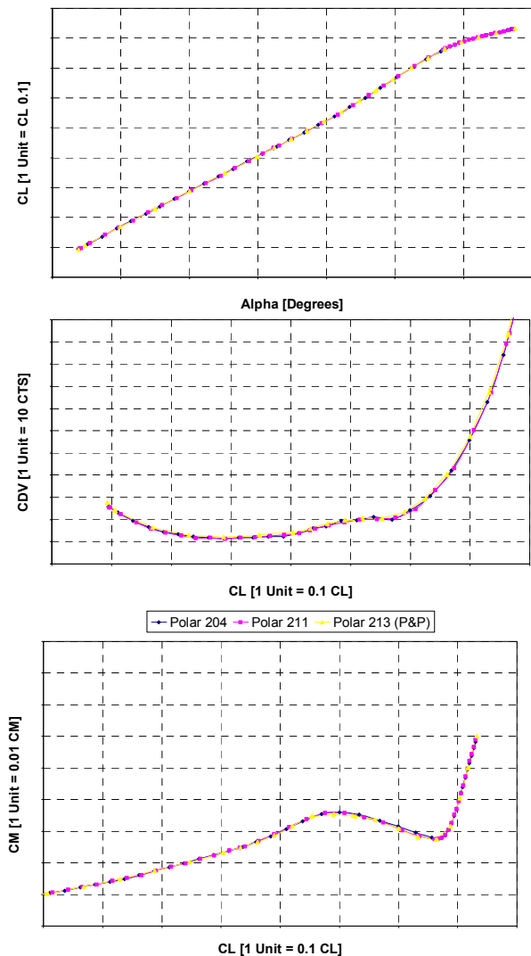
Figure 5 Short Term Repeatability – Forces Data
