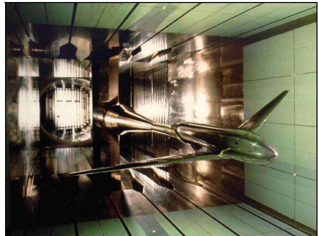
Figure 1 Model in the Test Section at ETW
